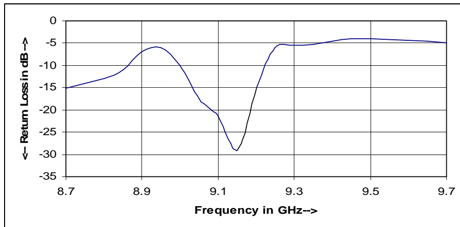
Figure 5: Simulated Return loss plot for antenna with taper at front (Figure 2)
