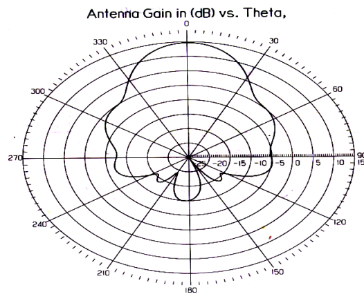
Figure 14: Radiation pattern for antenna 1 at \Phi = 0^\circ at resonant frequency
