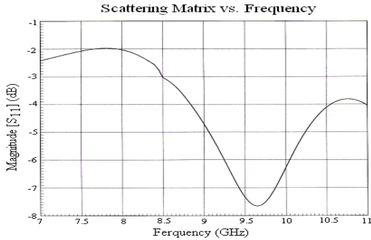
Figure13: Return loss pattern
