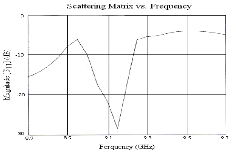
Figure 16: Return loss pattern for antenna
