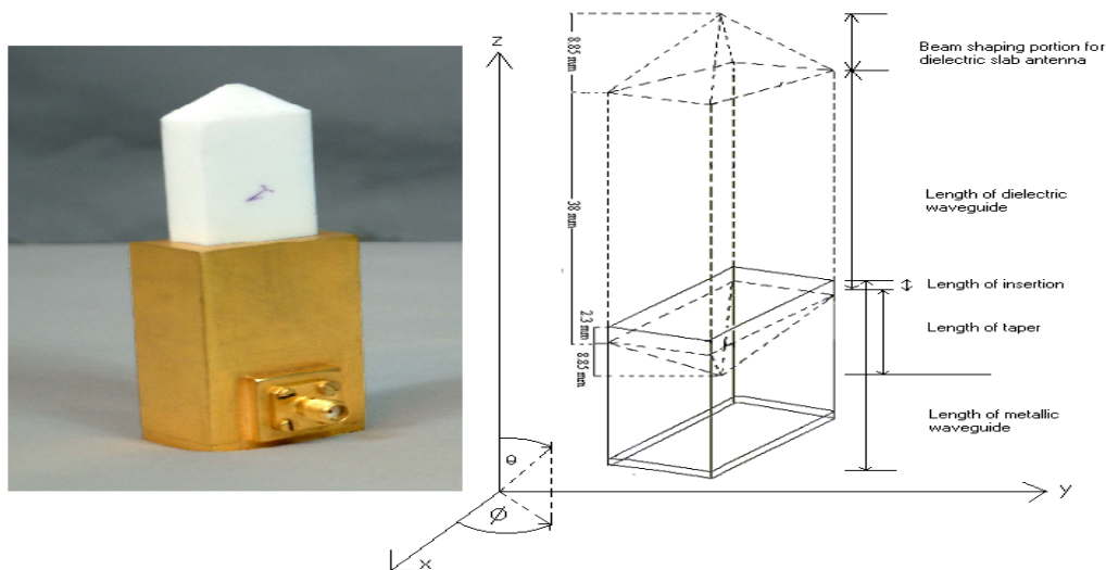
Figure 2: Dielectric Slab antenna with pyramidal matching section
