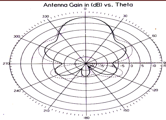
Figure 15: Radiation pattern for antenna 1 at — \Phi = 45^\circ and - - \Phi = 90^\circ at resonant frequency
