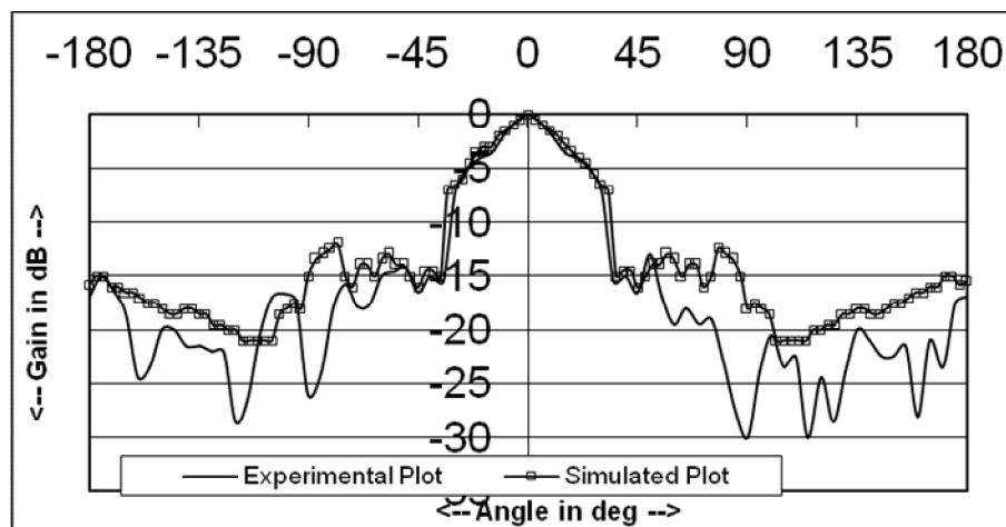
Figure 10: Simulated and experimental H filed radiation patterns for antenna with taper
