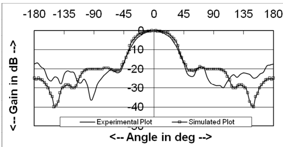
Figure 7: Simulated and experimental E filed radiation patterns for antenna without taper
