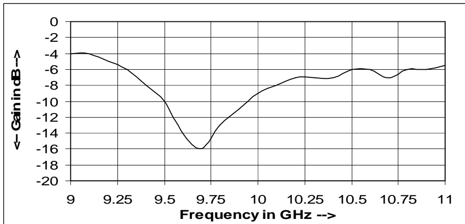
Figure 4: Measured return loss plot for antenna without taper at front
