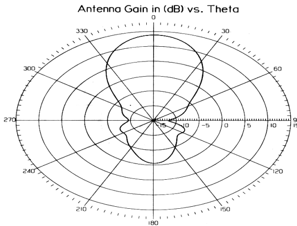
Figure 17: Radiation pattern for antenna 2 at \Phi = 0^\circ at resonance frequency
