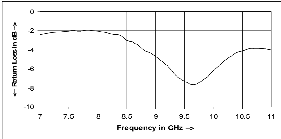
Figure 3. Simulated return loss plot for antenna without taper at front
