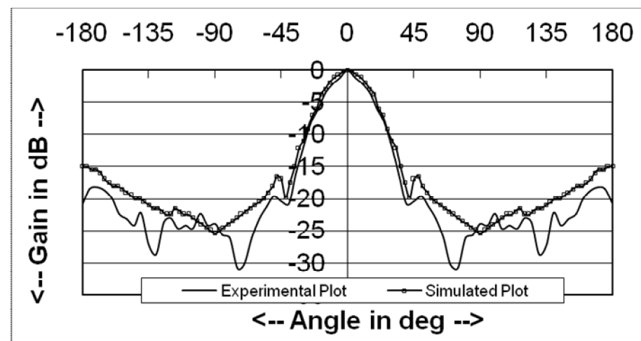
Figure 8: Simulated and experimental E filed radiation patterns for antenna with taper
