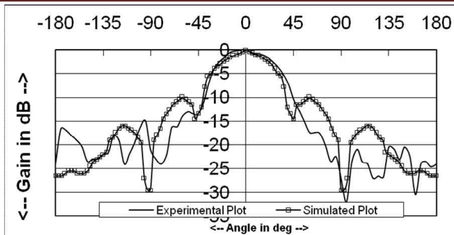
Figure 9: Simulated and experimental H filed radiation patterns for antenna without taper
