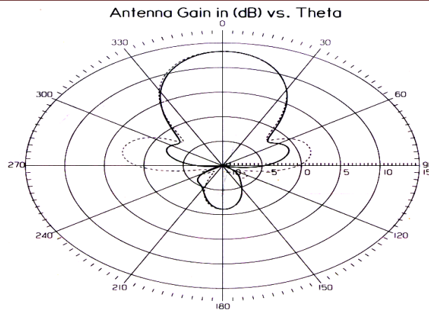
Figure 18: Radiation pattern for antenna 2. at — \Phi = 45^\circ and - - \Phi = 90^\circ at resonance frequency
