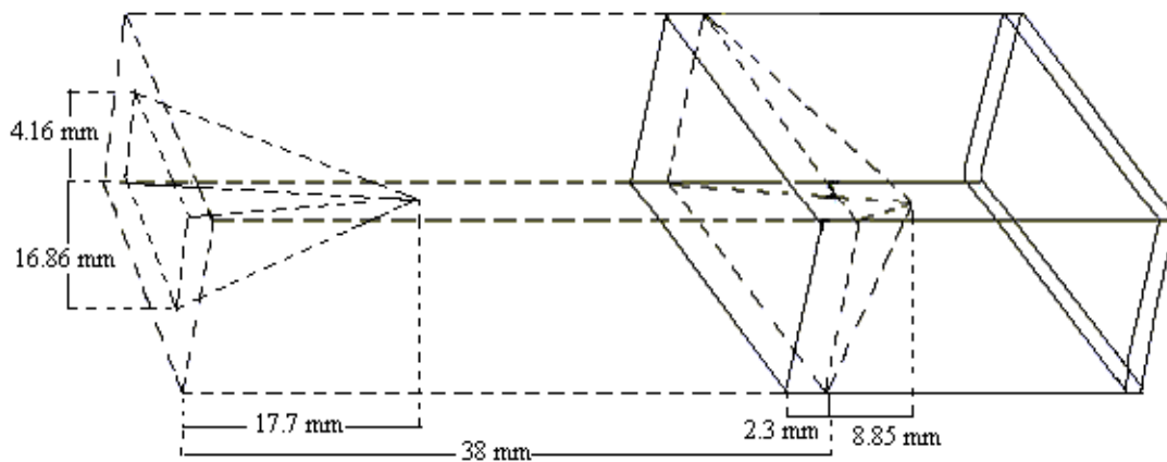
Figure 12: Dielectric slab antenna with pyramidal matching section and a hollow pyramid
