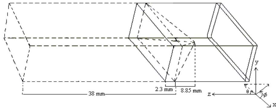
Figure 1. Dielectric slab antenna with pyramidal matching section (without front tapering)
