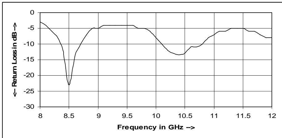
Figure 6: Measured return loss plot for antenna with taper at front (Figure 2)
