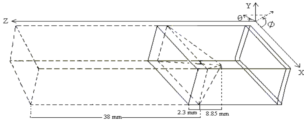
Figure 11. Dielectric slab antenna with pyramidal matching section
