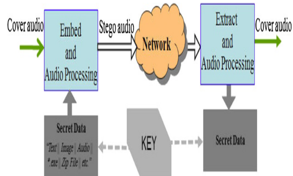
Fig 2: Audio Steganography
