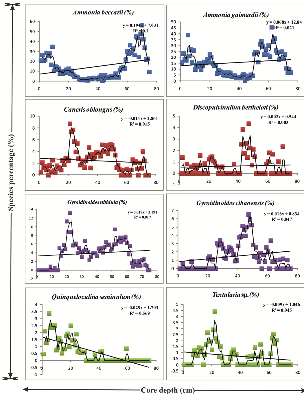
Figure 4: Scatter plot of percent distribution of benthic foraminiferal species against with core depth (cm) from Puthenthodu beach sediment, West coast of India.
