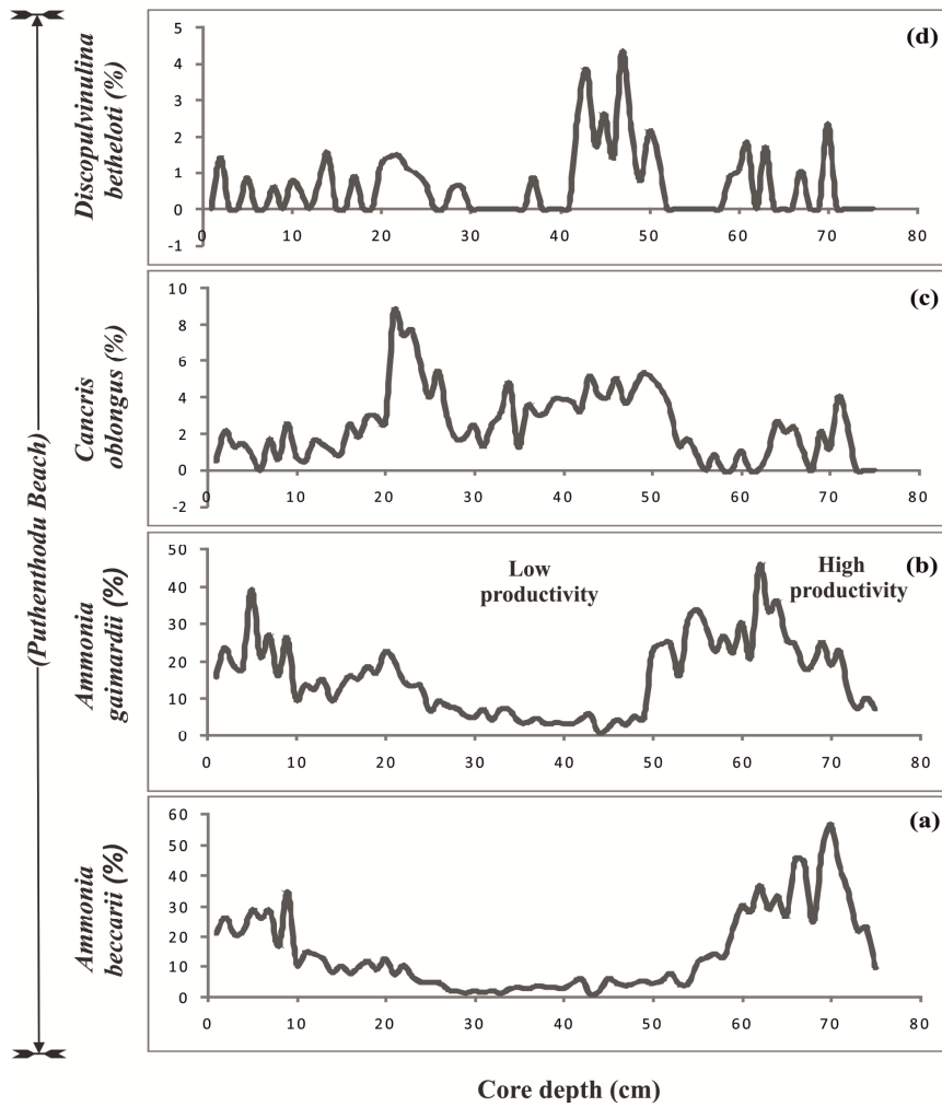
Figure 2: Percent distribution of benthic foraminiferal species Ammonia beccarii (panel a), Ammonia gaimardii (panel b), Cancris oblongus (panel c) and Discopulvinulina bertheloti (panel d) at Puthenthodu beach sediment, West coast of India.
