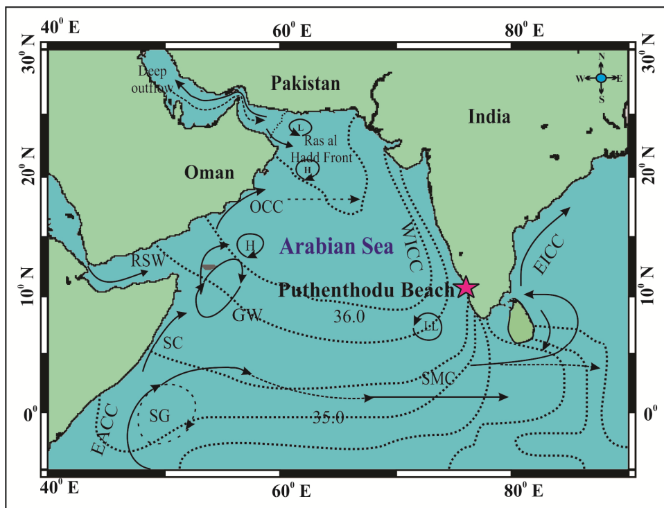
Figure 1: Location map showing core-sediment from Puthenthodu beach, West coast of India. Ocean currents prevalent during summer monsoon (Jul/Aug) indicated by solid/broken lines with arrows and annual sea surface salinity indicated by dotted lines, values in psu in the Arabian Sea.
