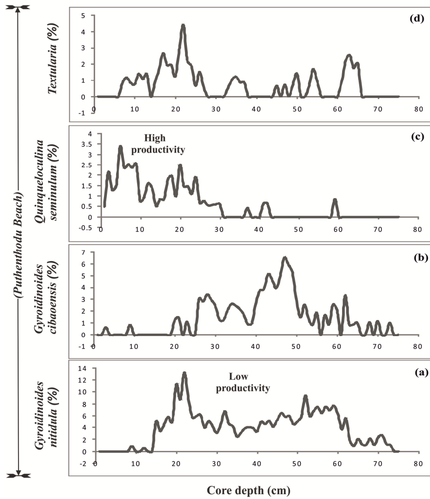
Figure 3: Percent distribution of dominant benthic foraminiferal species Gyroidinoides nitidula (panel a), Gyroidinoides cibaoensis (panel b), Quinqueloculina seminulum (panel c) and Textularia sp. (panel d) at Puthenthodu Beach sediment, West coast of India.
