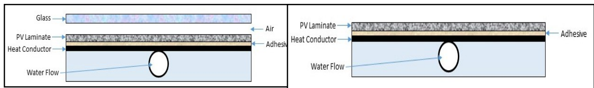
Figure3. Glazed Type Collector
