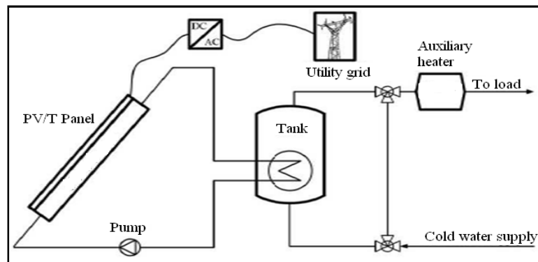
Figure2. Line Diagram of PVT System
