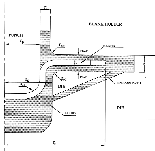
Fig.1 Hydro mechanical forming process
