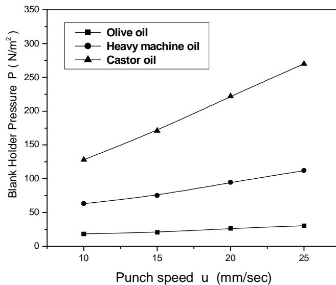
Fig.2 Blank holder force per unit area (Blank holder pressure) for different fluids
