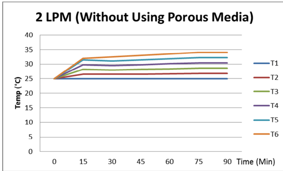
Fig.7. Time vs Temp Graph (2LPM)
