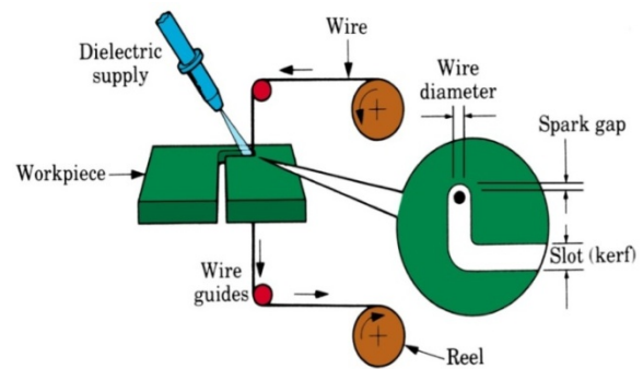
Figure 4- Machining process
