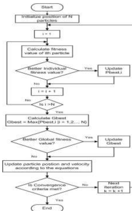
Fig 4:PSO flowchart
