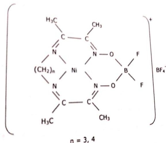
Figure - 2 The square planar geometry of [\text{Ni}(\text{H}_2 \text{Mahe}^{1-2})\text{BF}_2]\text{BF}_4 complexes.
