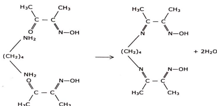
Figure – 1 - The chemical reaction of Synthesis of th ligands
