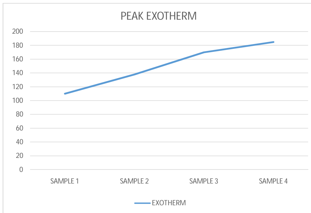
Figure 1 The above figure shows the gradual rise in Peak Exotherm as a higher glycol is used.
