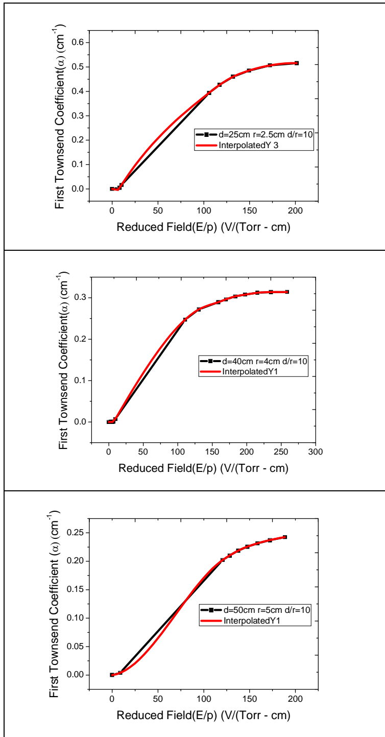
Figure 8: Interpolated graphs for first Townsend coefficient ( \alpha ) with E/p to obtain the variation of plots in the whole range
