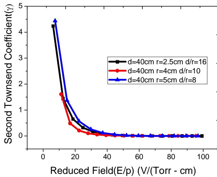
Figure 15: Variation of Second Townsend Coefficient ( \gamma ) as a function of E/p over a range of 0-100 V/(Torr-cm)
