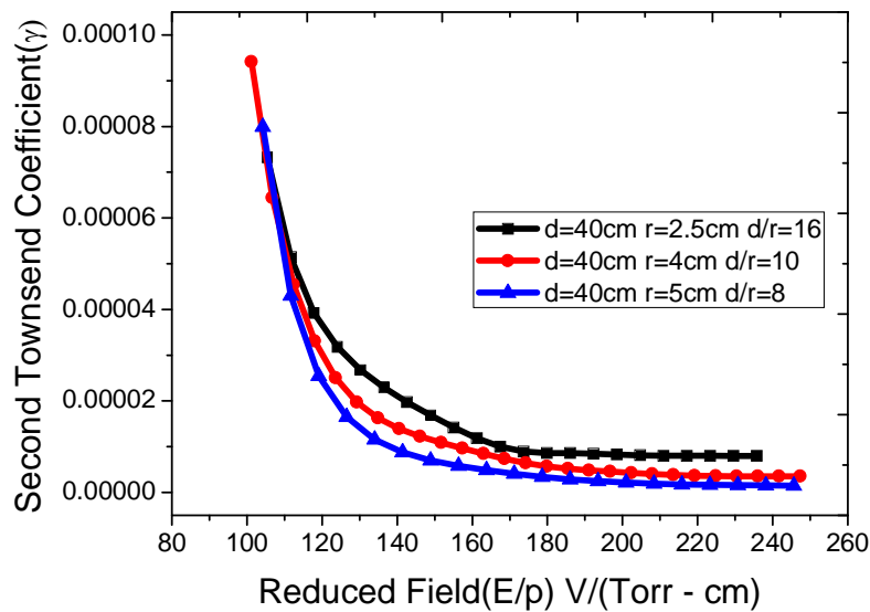
Figure 16: Variation of second Townsend coefficient ( \gamma ) as a function of E/p over a range of 100-250 V/(Torr-cm)
