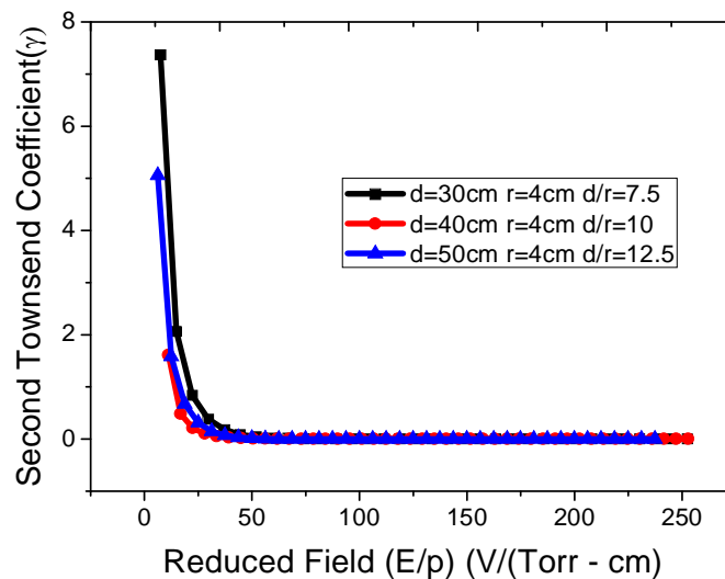
Figure 11: Variation of second Townsend coefficient ( \gamma ) as a function of E/p for different distances
