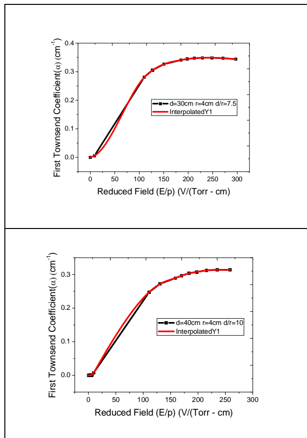
Figure 1: Variation of first Townsend coefficient ( \alpha ) with (E/p) for variable inter-electrode distances
