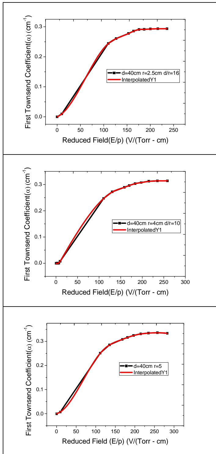
Figure 5: Interpolated graphs for first Townsend coefficient ( \alpha ) with E/p to obtain the variation of plots in the whole range
