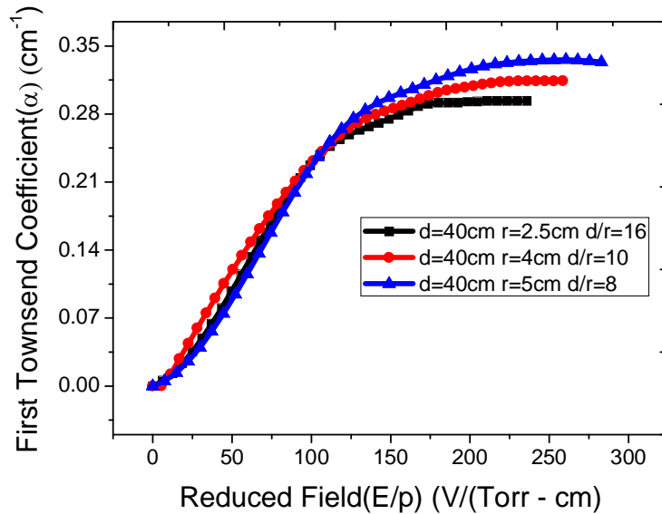
Figure 6: Variation of first Townsend coefficient ( \alpha ) with (E/p) for variable radius with whole range of E/p
