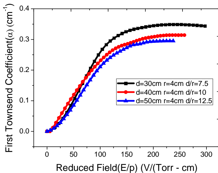
Figure 3: Variation of Townsend coefficient ( \alpha ) with ( E/p ) for variable distance with whole range of E/p
