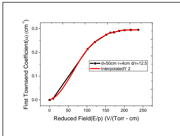
Figure 2: Interpolated graphs for first Townsend coefficient ( \alpha ) with E/p to obtain the variation of plots in the whole range
