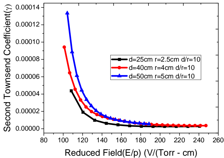
Figure 19: Variation of Second Townsend Coefficient ( \gamma ) as a function of E/p over a range of 100-250 V/(Torr-cm)
