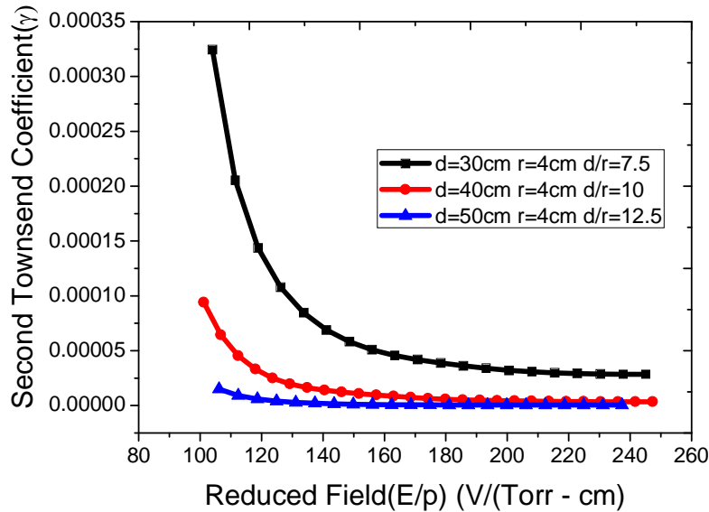
Figure 13: Variation of second Townsend Coefficient ( \gamma ) as a function of E/p over a range of 100-250 V/(Torr-cm)
