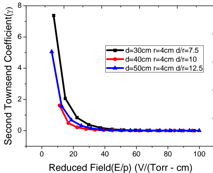
Figure 12: Variation of second Townsend coefficient ( \gamma ) as a function of E/p over a range of 0-100 V/(Torr-cm)
