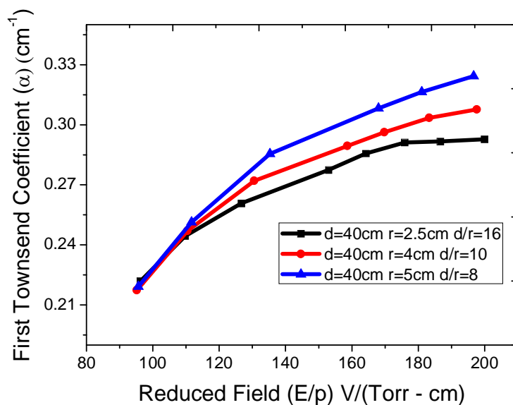
Figure 4: Variation of Townsend coefficient ( \alpha ) with (E/p) for variable electrode radius
