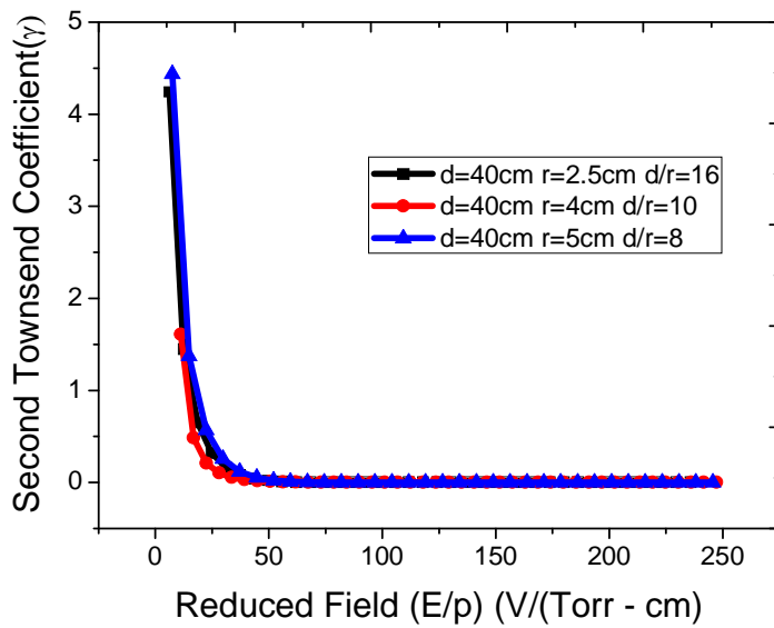
Figure 14: Variation of Second Townsend Coefficient ( \gamma ) as a function of E/p for different radius
