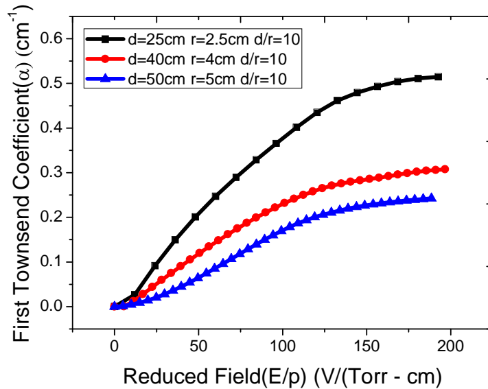
Figure 9: Variation of Townsend coefficient ( \alpha ) with (E/p) for constant d/r ratio for whole range of E/p
