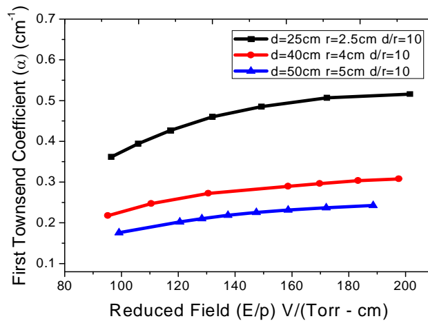
Figure 7: Variation of first Townsend coefficient ( \alpha ) with E/p for constant d/r ratio
