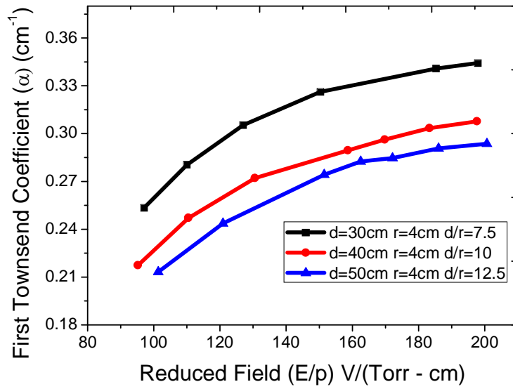
Figure 1: Variation of first Townsend coefficient ( \alpha ) with (E/p) for variable inter-electrode distances
