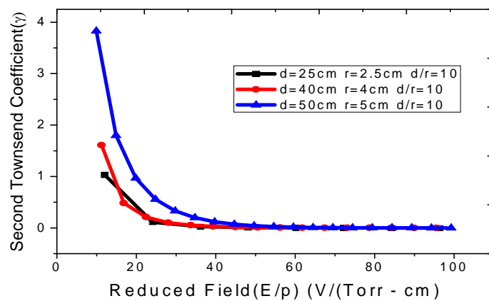
Figure 18: Variation of second Townsend coefficient ( \gamma ) as a function of reduced field E/p over a range of 0-100 V/(Torr-cm)
