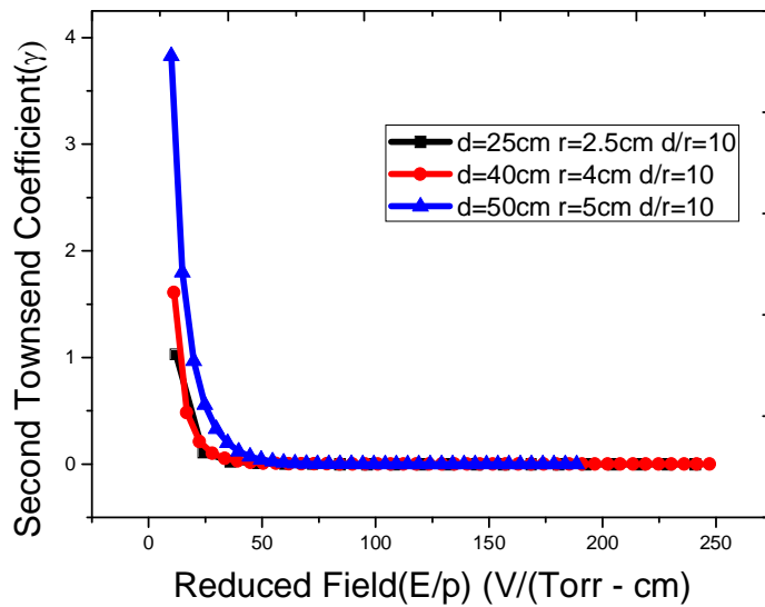
Figure 17: Variation of second Townsend coefficient ( \gamma ) as a function of reduced field E/p with constant d/r
