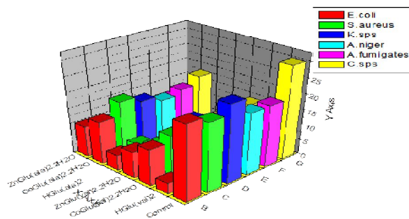
Fig .7: Antimicrobial activities of Schiff base ligands and its complexes by disc diffusion method (Zone inhibition in mm)
