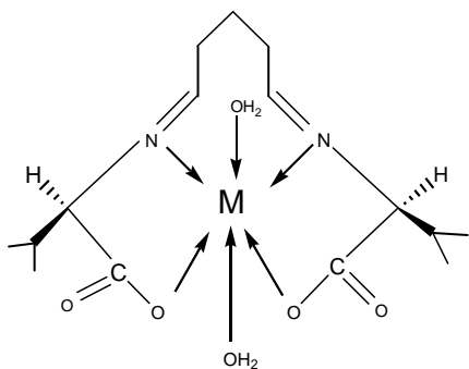
Fig .8: Structure of HGlu(val) 2 complexes
