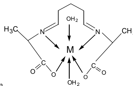
Fig.9: Structure of HGlu(ala) 2 complexes
