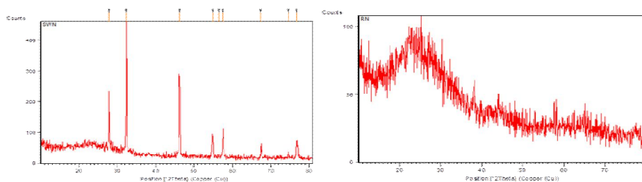
Fig. 3: Powder XRD pattern of the CoGlu(val) 2 .2H 2 O and ZnGlu(val) 2 .2H 2 O complexes
