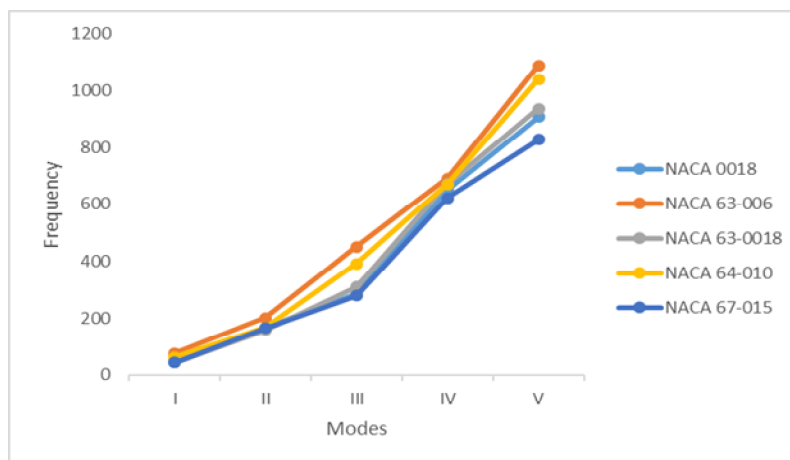
Fig. 2 Variation of frequency with modes
