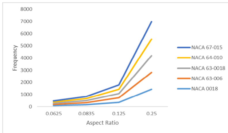
Fig. 4. Variation of vibration frequency in second mode with aspect ratio.
