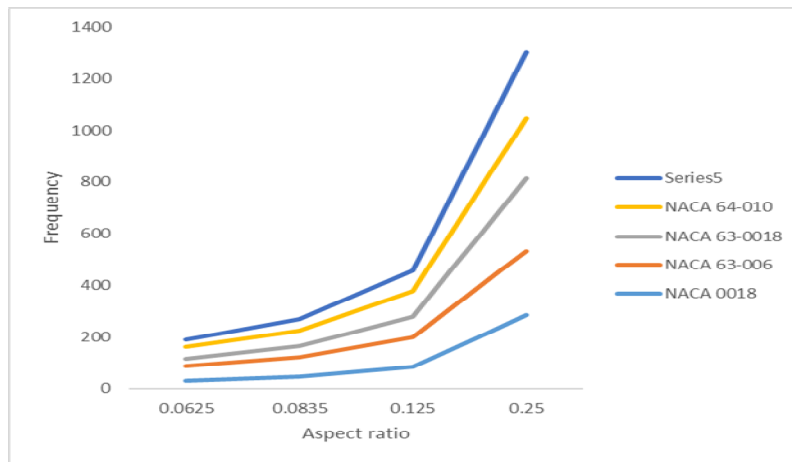
Fig. 3 Variation of vibration frequency in fundamental mode with aspect ratio.
