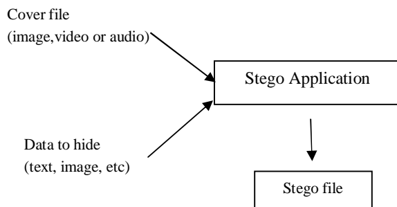
Fig 1: Steganography
