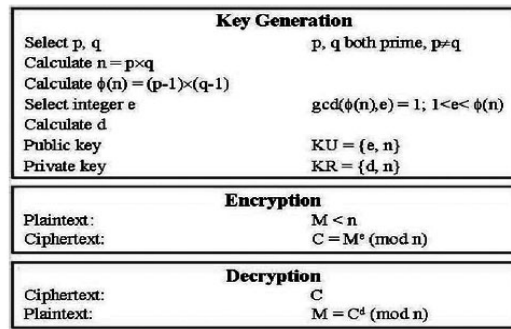
Fig 3: RSA Algorithm
