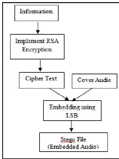
Fig 4: LSB Encoding
