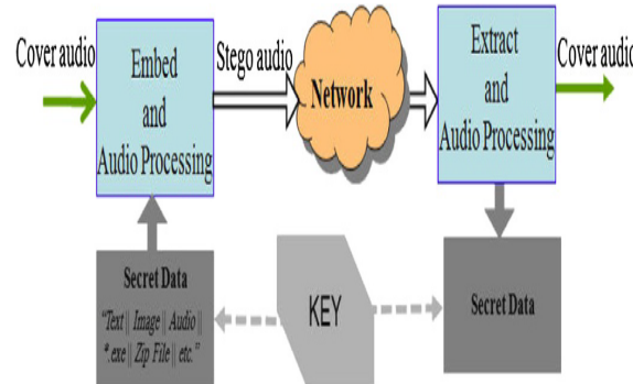
Fig 2: Audio Steganography
