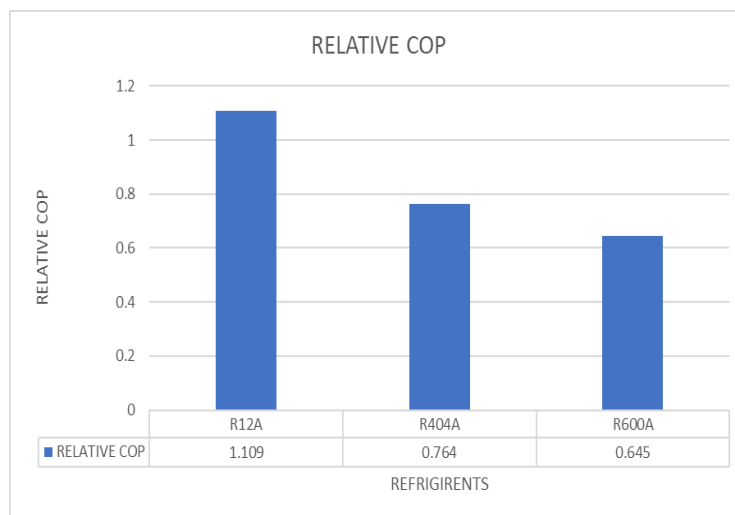
Fig 4: Comparison between Relative cop of the Refrigerants
