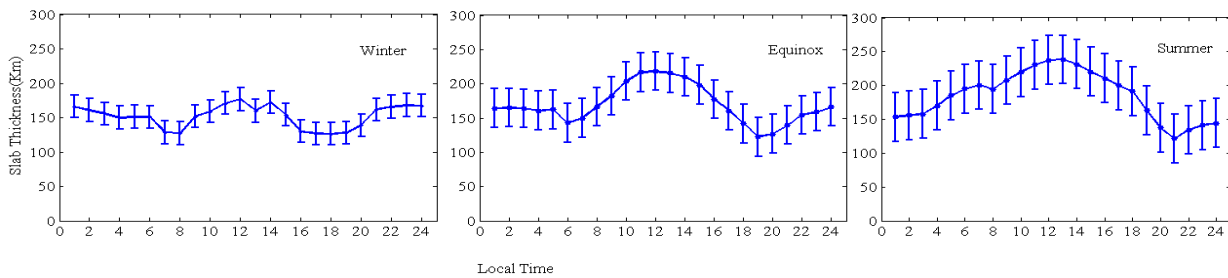
Figure2: Seasonal variation of slab thickness during August, 2011-July, 2012.
