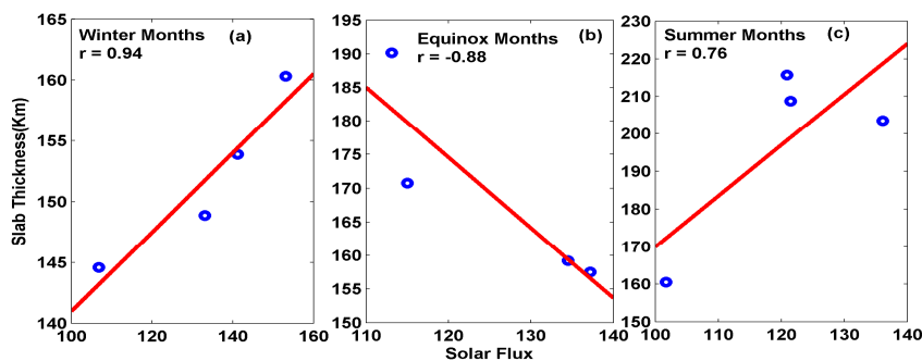
Figure3: Solar activity variation of slab thickness during August, 2011- July, 2012
