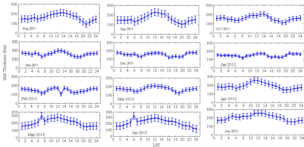
Figure 1: Diurnal profile of monthly mean values of seasonal for each month with standard deviation bar from August, 2011 – July, 2012.
