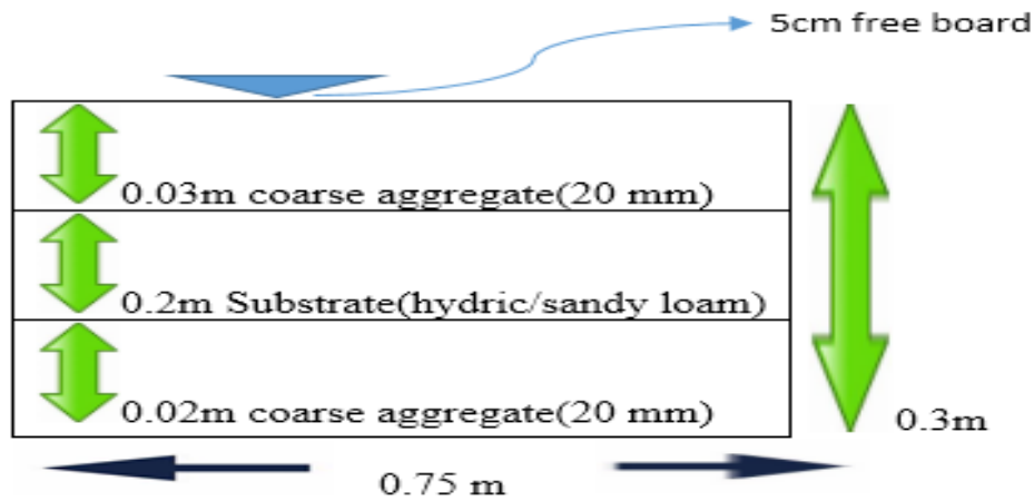
Figure -1: Line diagram of model showing different layers
