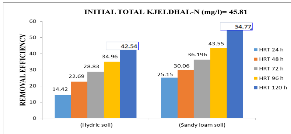
Figure -14: Removal efficiencies of Total Kjeldhal Nitrogen at various HRT
