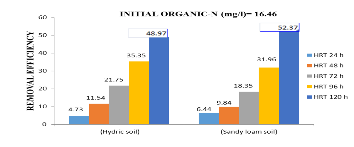
Figure -15: Removal efficiencies of Organic Nitrogen by VSSFCW Model at various HRT
