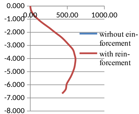
Chart2. Bearing capacity s/B % graph
