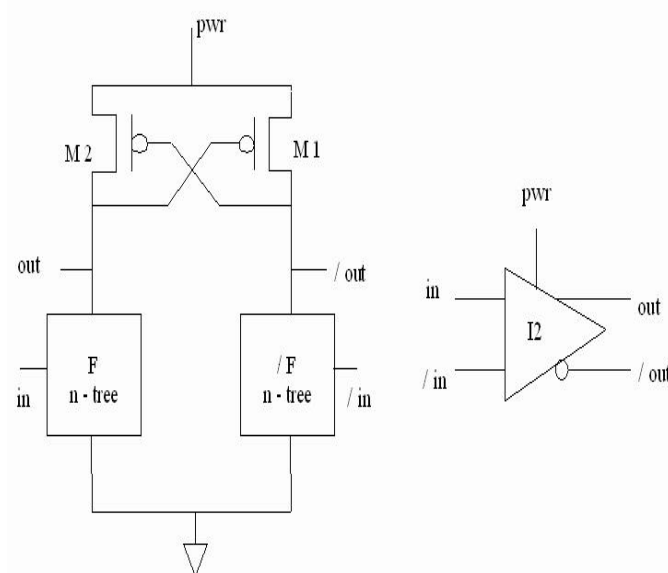
Figure 4.1. The Basic Structure of the Adiabatic ECRL Logic.
