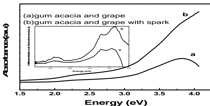
Fig. 4: UV-VIS spectrum of acacia gum, treated with black grapes of e-beam irradiated samples.
