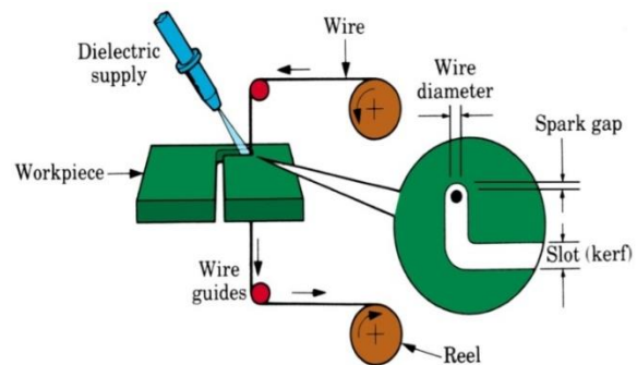
Figure 4- Machining process
