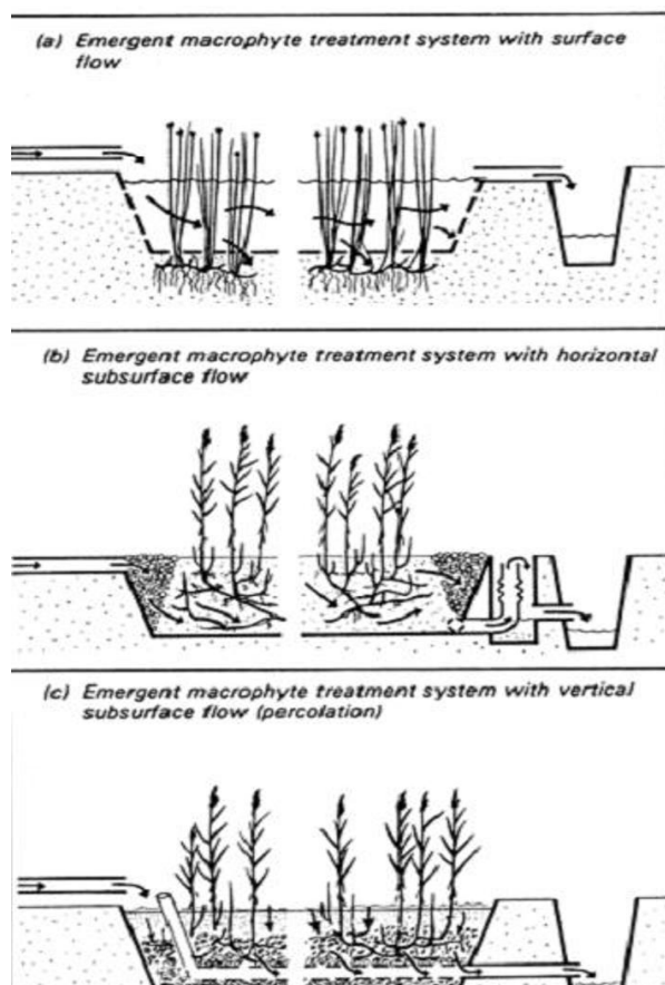
Fig. No. 1 : Three types of Constructed wetland 10
