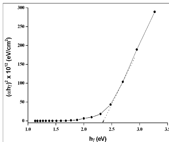
Fig. 6 Variation of (\alpha h\nu)^2 versus h\nu of the as-deposited CdO film
