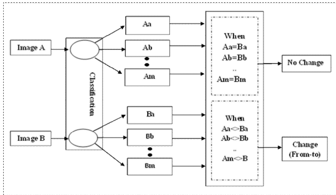
Figure 3: Flow diagram for change detection matrix
