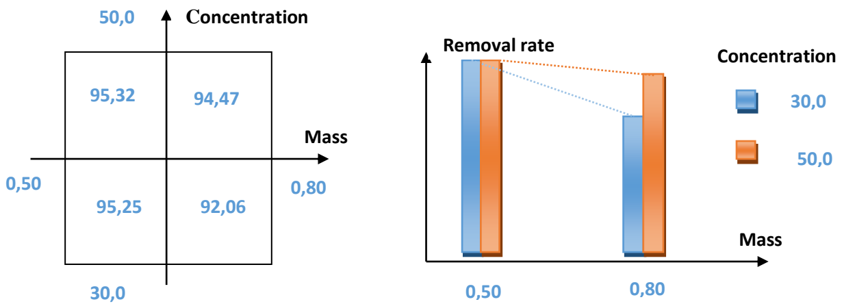
Figure 6 : Biosorbent mass interaction diagram–concentration (b 23 )
