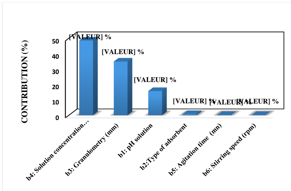
Figure 3: Pareto diagram of the Plackett and Burman design
