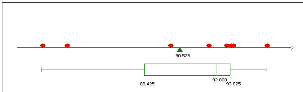
Figure 2: Diagram of the quartiles of the Hadamard design
