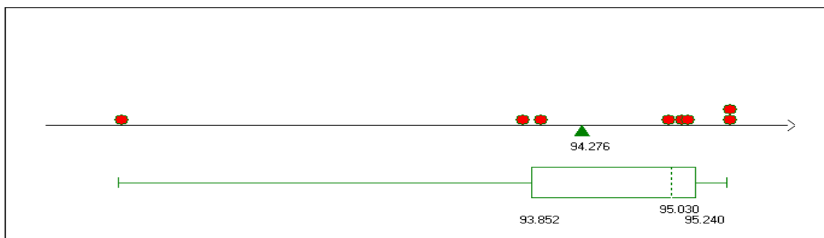
Figure 4: FD Quartile diagram
