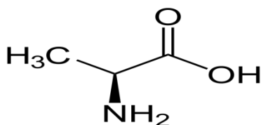
Figure 1. L-alanine structure.
